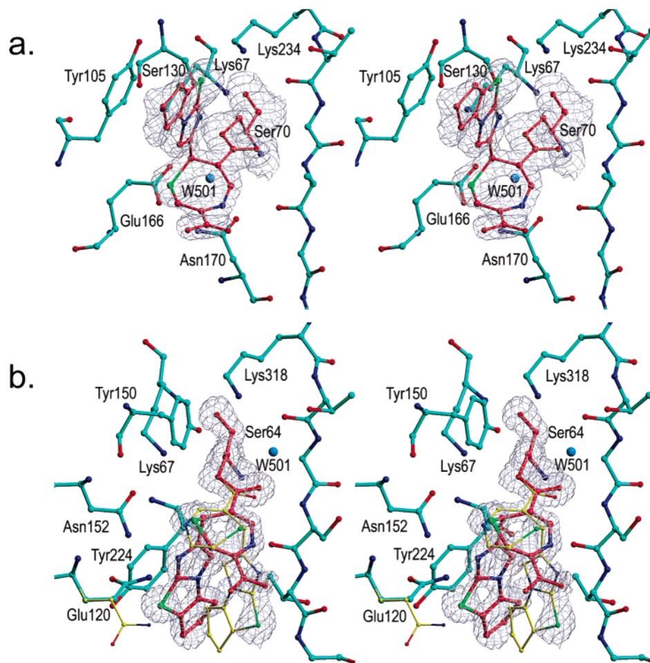
Figure 3. Stereoview of the F_o - F_c electron density of the intermediate 27 bonded to the reactive serine in (a) the SHV-1 \beta -lactamase and (b) the GC1 \beta -lactamase. The density contour level is 3\sigma . The figure was made by XtalView 18 and Raster3D. 38
